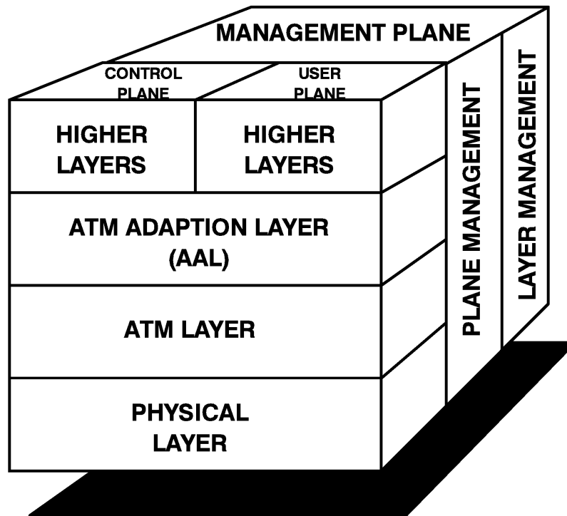
Figure 10.4 ATM Protocol Reference Model (PRM) [1]
