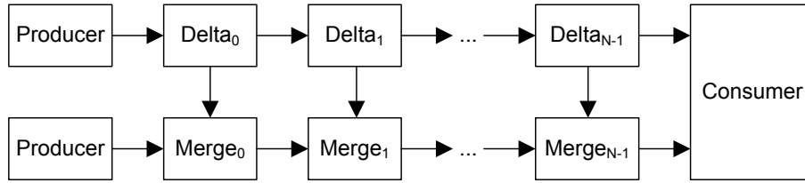
Figure 3. The twin pipeline benchmark: two producers, a dual consumer, and N connected delta and merge processes inbetween.
